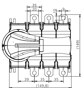
YCOT EHA C 315/315A 03
