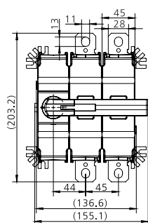
YCOT EHA B 630/400A 12
