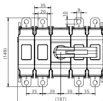
YCOT EHA B 315/160A 22
