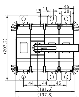
YCOT EHA B 630/400A 12
