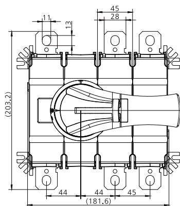
YCOT EHA C 630/400A 12
