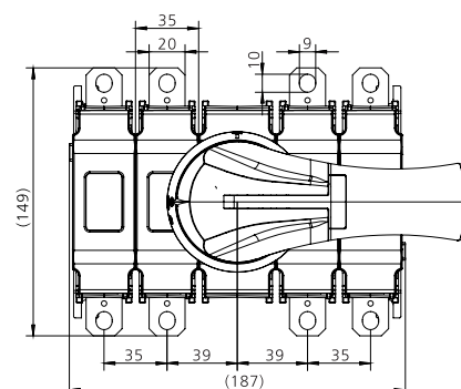
YCOT EHA C 315/160A 22
