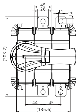
YCOT EHA C 630/400A 12
